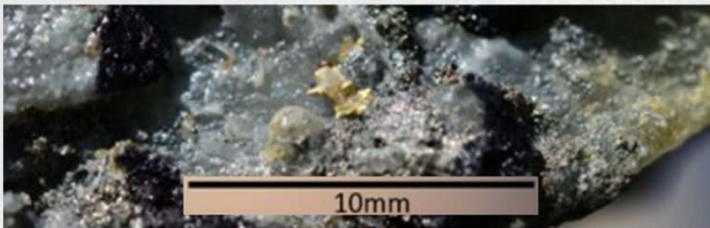
Quartz veinlet displaying coarse visible gold
